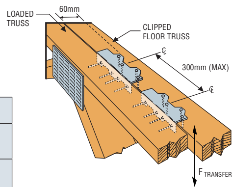
Typical L70 Installation
